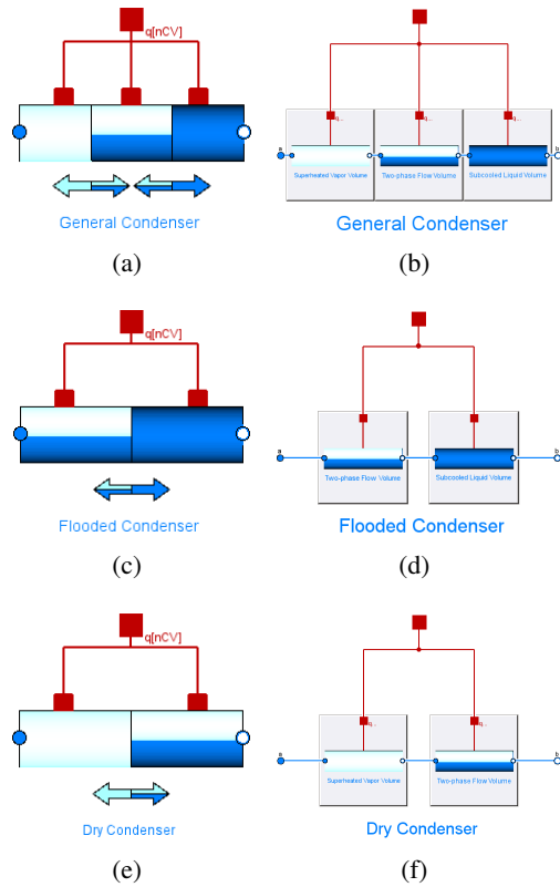
Figure 9: Condenser components
