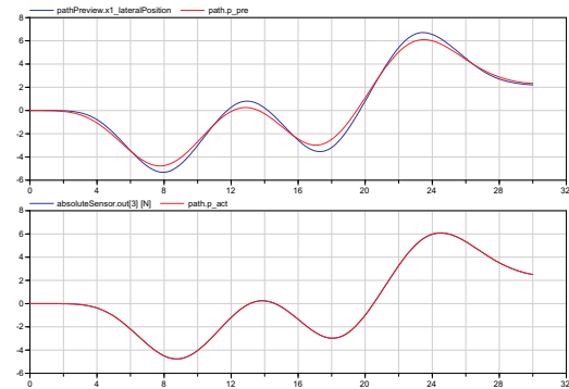
Figure 22: Simulation result of a motorcycle tracking a pre-defined path. Upper plot: The red signal is the path a pre-defined distance ahead, the blue signal is the preview distance of the rider. Lower plot: The red signal is the actual path, the blue signal is the traveled path measured at the rear frame's center of mass
