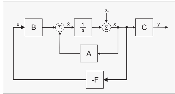
Figure 5: State feedback
