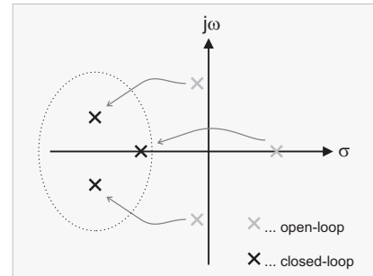
Figure 6: Graphical interpretation of the pole placement technique. Eigenvalues (poles) of the system located in the left-half plane correspond to stable behavior.
