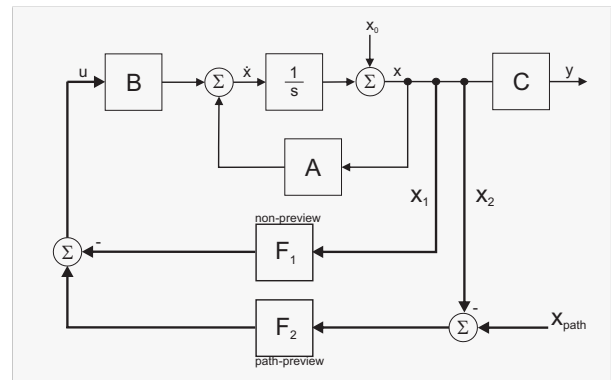
Figure 16: Basic structure of a state-space path preview controller. The state vector x_1 includes the states that are responsible for the stability (non-preview), whereas x_2 = (x_{lat} \dot{x}_{lat})^T includes the states required for path tracking.
