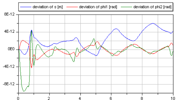
Figure 5: Deviations between both simulations for trolley position s and both angles \varphi_1 and \varphi_2
