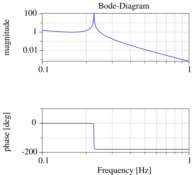
Figure 10: Bode-Diagram of the spur gear from Figure 6
