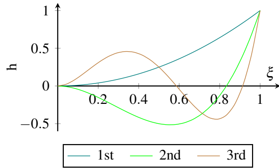
Figure 4: shape functions for v and w
