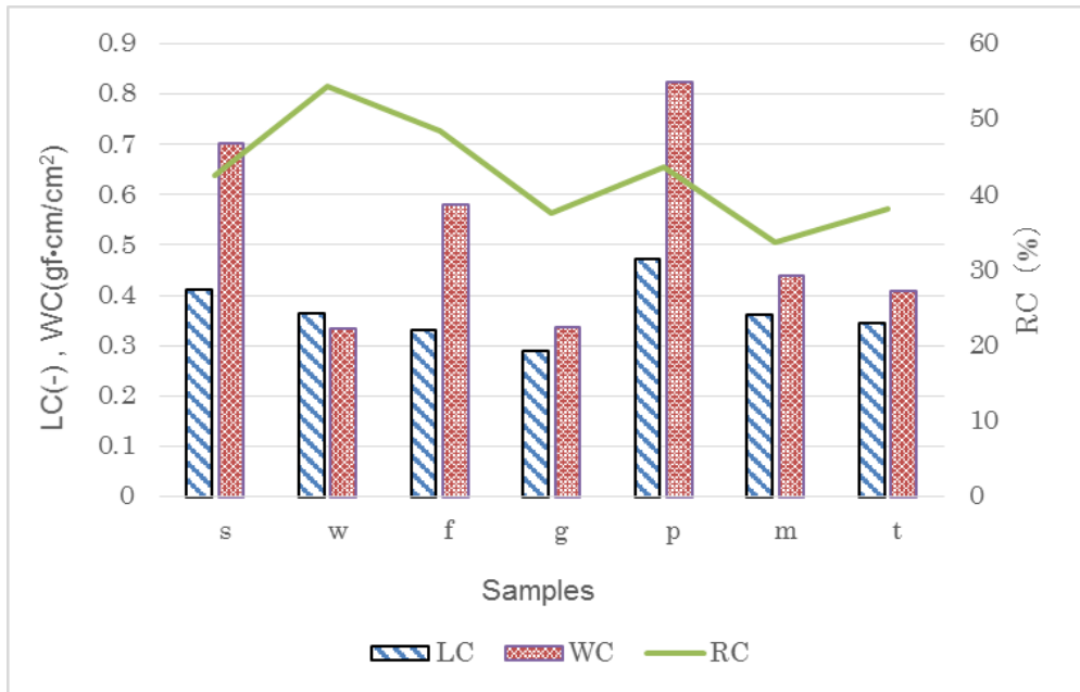
Figure 2: Compression properties measured
