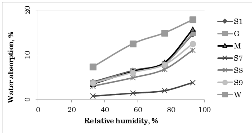
Figure 4: The changes of water absorption
