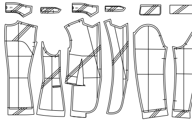
Figure 1: Jacket pattern with interlining parts (diagonal lines)
