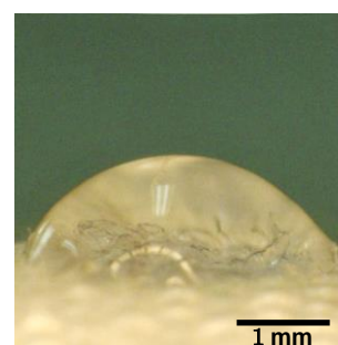
Fig.3 Photograph of the water droplet on the cotton fabric that was immersed in 5 \times 10^{-4} mol/L stearylamine benzene solution.
